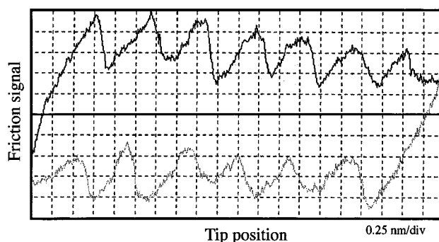
Figure 7. A typical LFM scope trace showing a friction loop. Scanning proceeds from left to right on the top line (trace) and from right to left following the bottom line (retrace). One division on the y axis corresponds to 0.02 V friction signal. Scanning was performed at 66.3° with respect to the chain direction.
