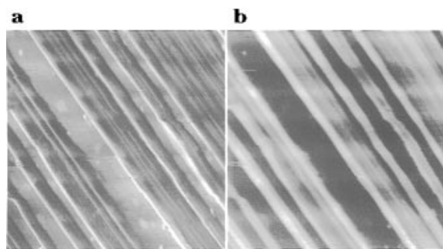
Figure 4. Lateral force microscopy (a) and contact-mode (height) atomic force microscopy (b) images of PTFE deposited on muscovite mica. The same area of 1\ \mu\text{m} \times 1\ \mu\text{m} is depicted on both micrographs.
