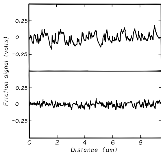
Figure 3. Cross-section plots of the lateral force microscopy signal shown in Figures 1a and 2a at a distance of ca. 2\ \mu\text{m} from the bottom edge of the LFM images, obtained in the horizontal ( \times ) direction. Top figure: first scan; bottom figure: third scan.
