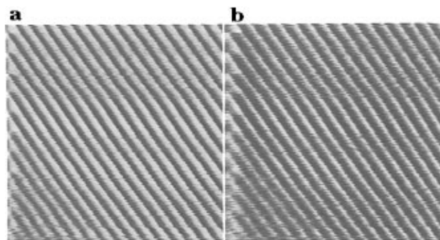
Figure 5. Dual-mode lateral force microscopy (a) and contact-mode (height) atomic force microscopy (b) images of PTFE deposited on muscovite mica showing molecular resolution. Scan size: 10.7\ \text{nm} \times 10.7\ \text{nm} ; the same area is shown in both images. Scan direction: 55° with respect to the chain direction.
