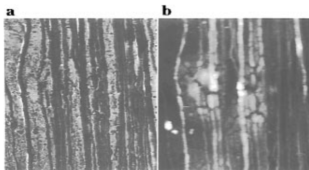
Figure 1. Lateral force microscopy (a) and contact-mode (height) atomic force microscopy (b) images of PTFE deposited on glass. The same area of 9.5 μm × 9.5 μm is depicted on both micrographs; first scan.
