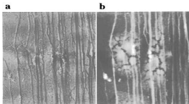
Figure 2. Lateral force microscopy (a) and contact-mode (height) atomic force microscopy (b) images of PTFE deposited on glass (same area that is shown in Figure 1; third scan). Scan size: 9.5 μm × 9.5 μm.
