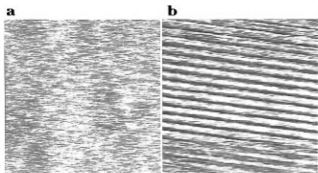
Figure 6. Dual-mode lateral force microscopy (a) and contact-mode (height) atomic force microscopy (b) images of PTFE deposited on muscovite mica. Scan size: 10 nm \times 10 nm; the same area is shown in both images. Scan direction: 6° (nearly parallel) with respect to the chain direction.
